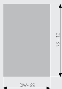
3. Wooden Drawer Bottom
